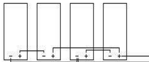
Two 12v/3.5A panels in series and two in parallel. This doubles the voltage and doubles the amps to make 24 volts and 7 amps.
